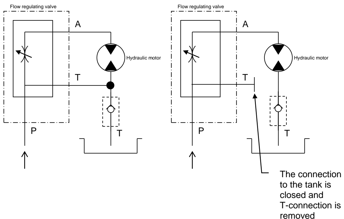
Standard "Open" hydraulic system
